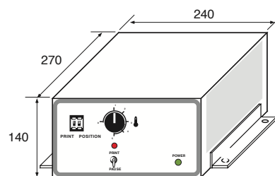
CONTROL UNIT
