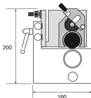
PRINTER DIMENSION
